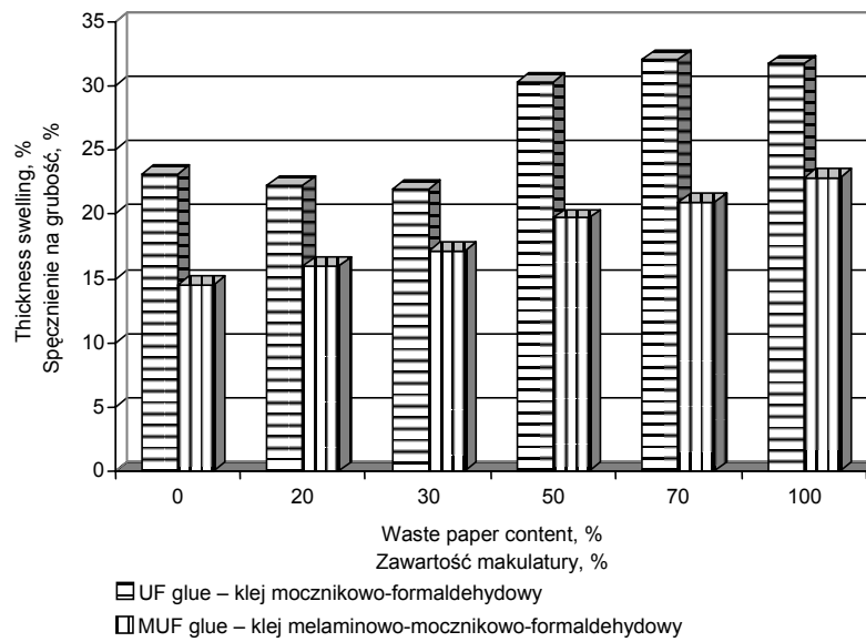
Fig. 7. Changes in the thickness swelling of boards in relationship to content of particles of mixed waste paper
