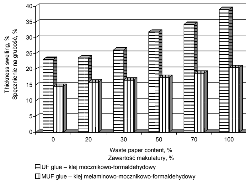
Fig. 8. Changes in the thickness swelling of boards in relationship to content of particles of waste paper bags
