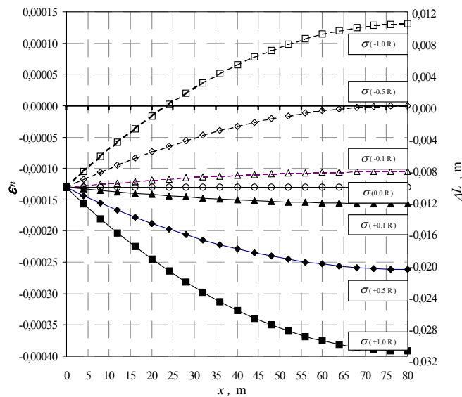
Fig. 10. Values of strains \epsilon_n(x,y) in the shell of cylindrical plywood made of birch with R = 0.75 , t = 0.5 , L = 80 m
